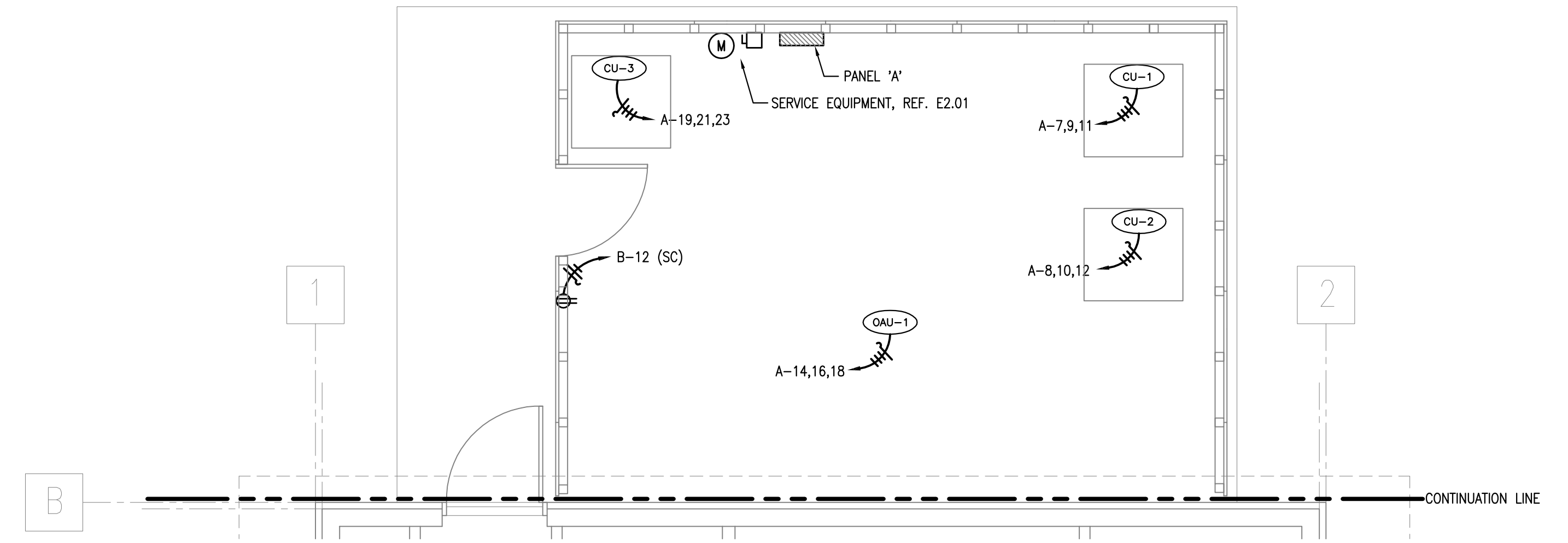
2 ELECTRICAL EQUIPMENT YARD SCALE: 1/4" = 1'-0"
