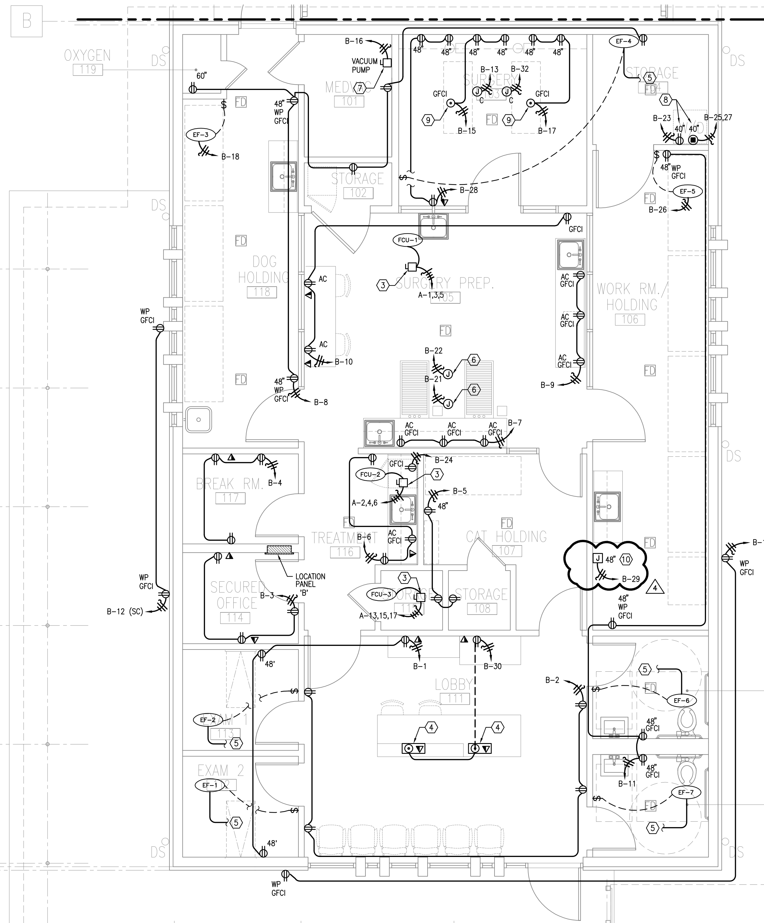
1 ELECTRICAL POWER FLOOR PLAN SCALE: 1/4" = 1'-0"
