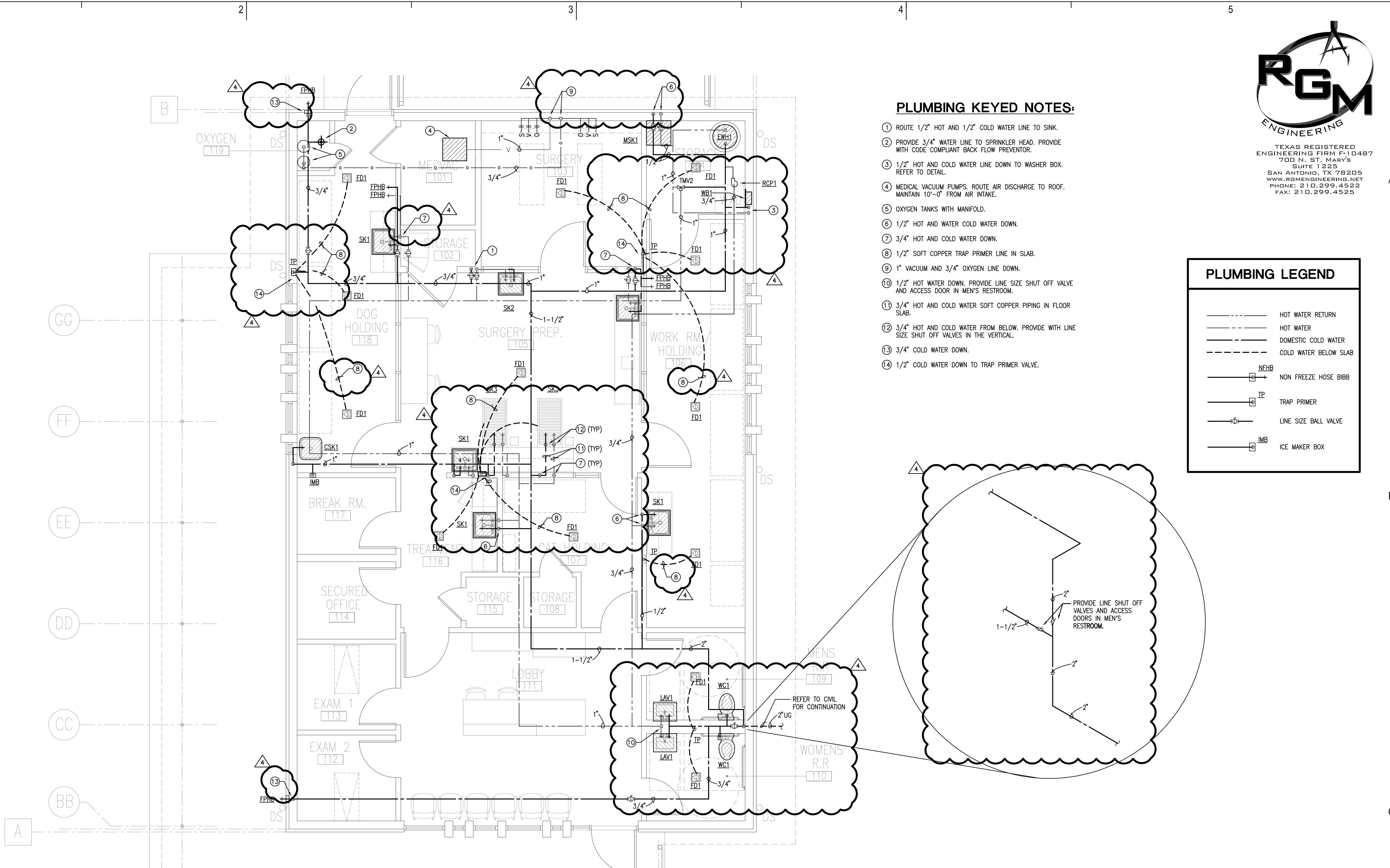
1 PLUMBING DOMESTIC WATER AND MEDICAL GAS FLOOR PLAN SCALE: 1/4" = 1'-0"
